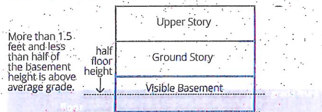
Visible Basement Diagram
